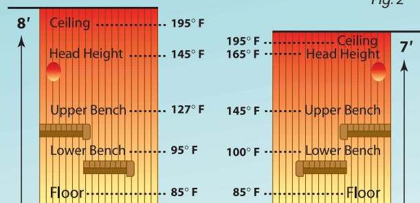
Incorrect Ceiling Height
